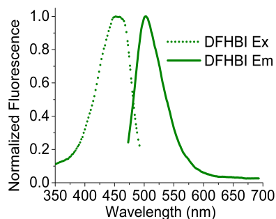
Figure 2. Excitation and emission spectra of Spinach ™ /DFHBI complex.
